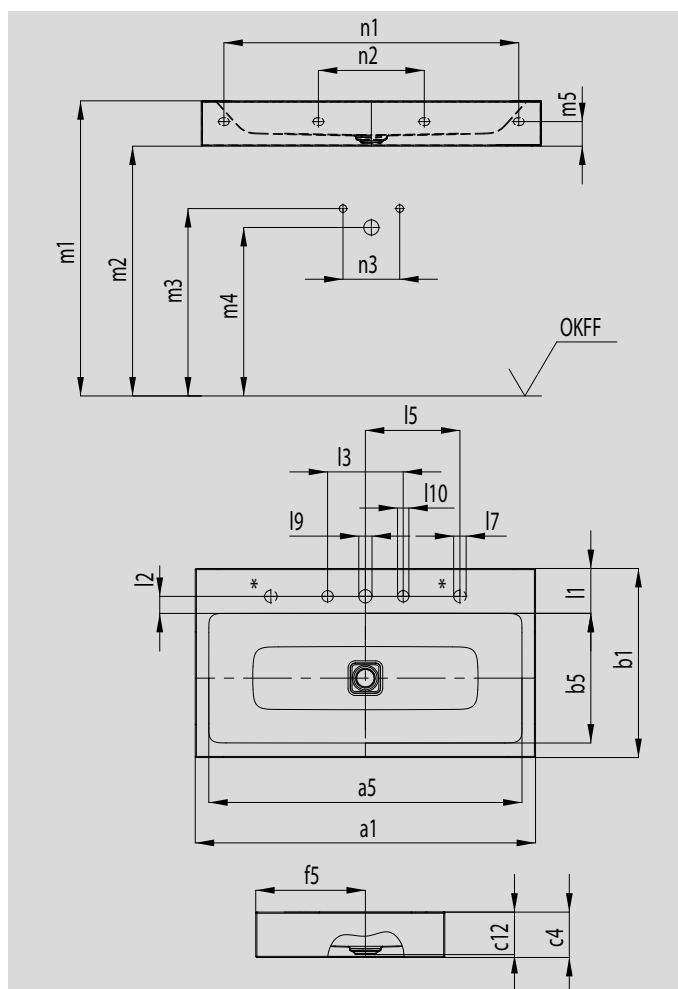
* Control knob holes for CLOU waste and overflow system with cable operated pop-up waste and deck mounted control knob
