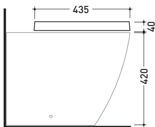
art. LK117 vista laterale / lateral view
