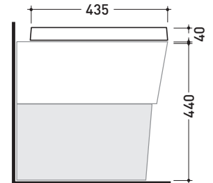
art. 5064A vista laterale / lateral view
