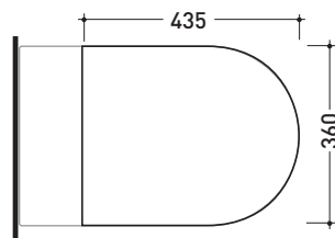
art. 5051/WC vista zenitale / zenital view
