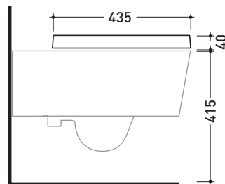
art. 5051/WC vista laterale / lateral view
